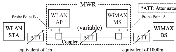
Fig. 4 Block diagram of mutual interference.
