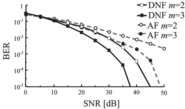
Fig. 4 BER of AF and DNF.
