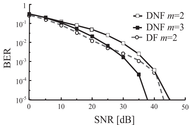
Fig. 5 BER of DF and DNF.
